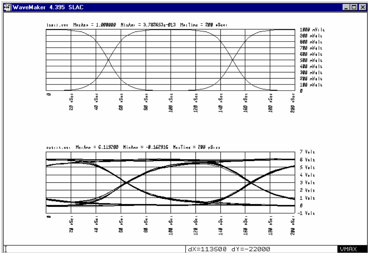
The corresponding “EYE” diagrams for the input and output waveforms.
