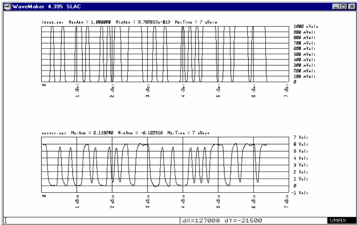
The input and output 10 Gbit/sec NRZ PRBS waveforms.
